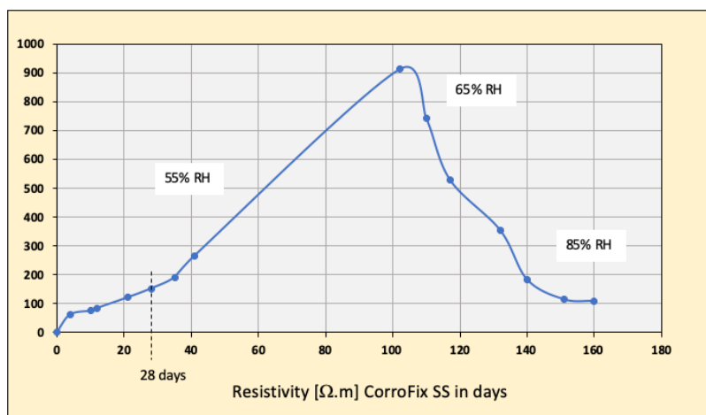
1. Course of resistivity ( \Omega m ) over time at different relative humidities (% RH)
