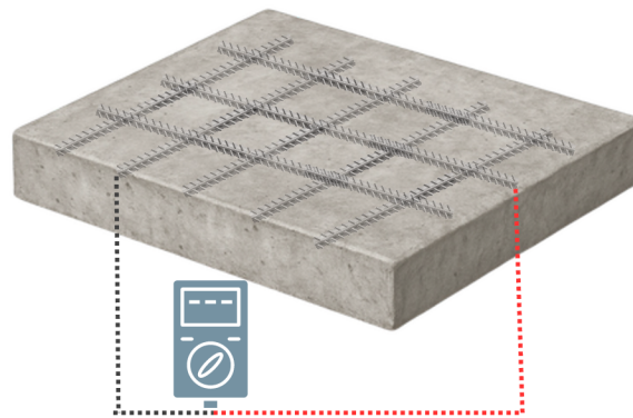
Check electric continuity of the reinforcement
